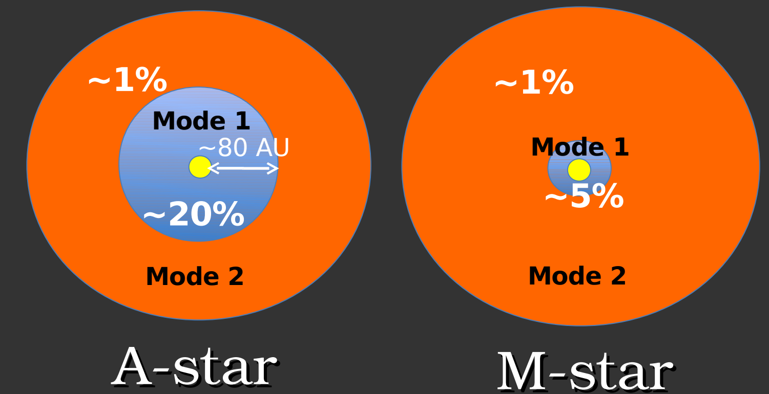
Fig. 5 - The simplest explanation for all exoplanet images to date: two modes of formation. Companions that form close to their star exhibit very strong correlations between star mass and planet properties: planet occurrence rate, semimajor axis extent, and mass all rise with increasing star mass. Mode 1 (blue region) is likely "core-accretion" and is also responsible for creating the Doppler RV planet population. Another mechanism, Mode 2 (orange region) has a lower occurrence rate at wide separations. Our simulations indicate that companions with ultra-wide orbits may exhibit very little correspondence between star mass and planet properties.
