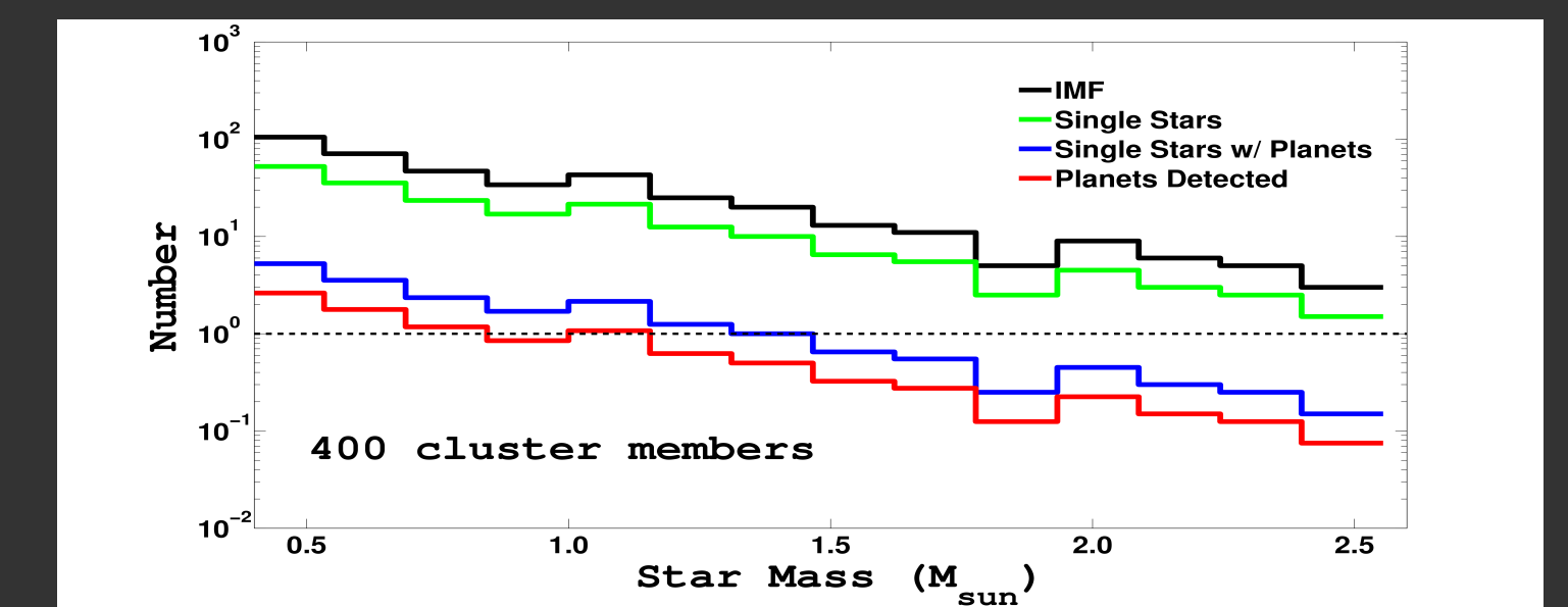
Fig. 6 - The number of detections in a (tightly bound) young stellar cluster always favors low-mass stars (see Fig. 4). Since the stellar IMF falls off faster than the planet occurrence rate grows, MK stars are the first spectral-types to produce planet images. This bias is exacerbated by the fact that: (i) half of star systems are binaries and high-contrast teams avoid binaries; (ii) the youngest stars are at a distance of \sim 140 pc, forcing the overall planet occurrence rate to take on its value at wide separations; (iii) the occurrence rate of ultra-wide separation planets appears to be only several percent.
