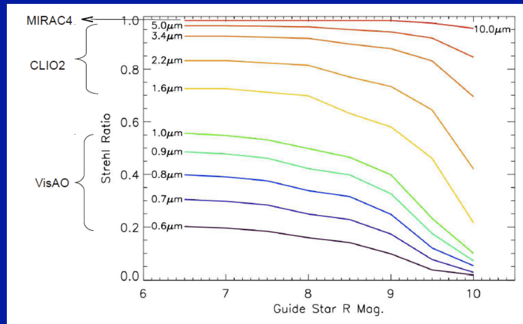
Simulated Performance of the Magellan AO System
